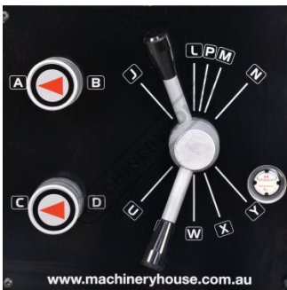
Feeds and Threads Gearbox Levers
