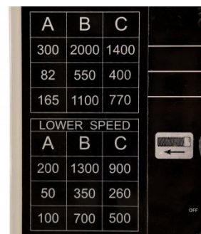
Spindle Speed Chart
