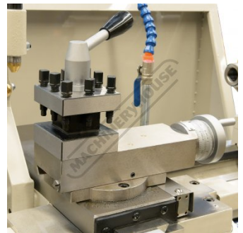
4-Way Toolpost
