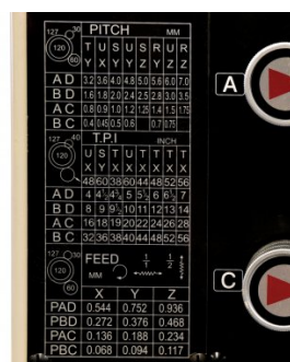
Thread-Feed Chart
