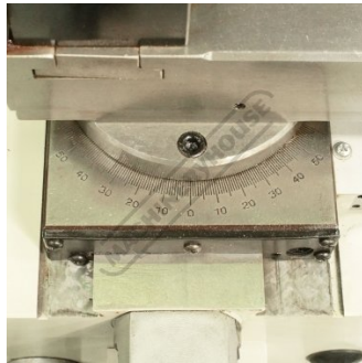
Compound Slide Scale
