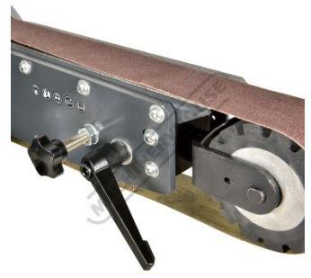
Belt Tensioner Adjustment
