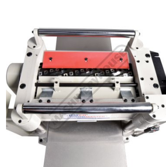
Five Spiral Cutter Head Top View
