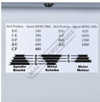
Speed Chart
