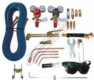
Oxygen Acetylene Gas Kit Contents
