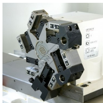
6 Station Tool Changer
