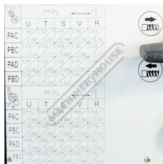
Screw Charts
