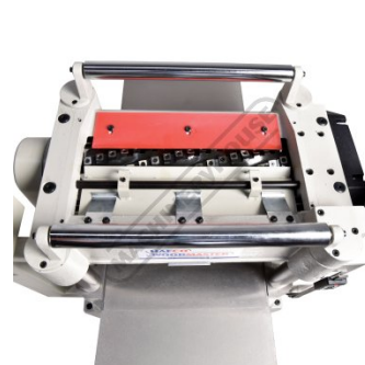
Five Spiral Cutter Head Top View
