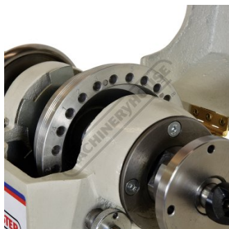
24 Position Indexing
