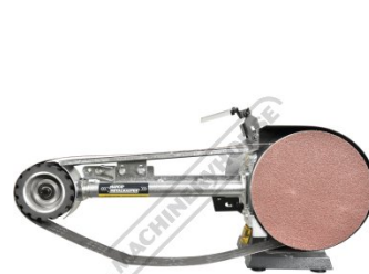
Adjustable Belt Tensioner
