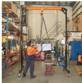
Shown Lifting Oil Tank
