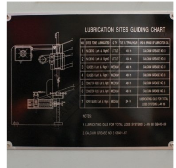
Lubrication Chart
