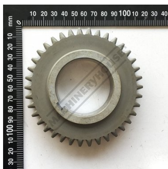
1 Top View
