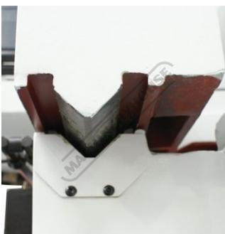
Large Table Vee Slide with Turcite B Coating
