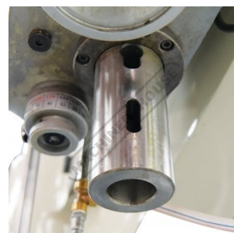
5MT Spindle
