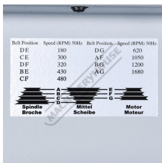
Speed Chart
