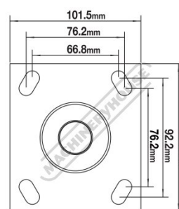
Baseplate dimensions Baseplate Dimensions
