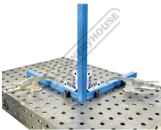
Square Tube Setup with Optical Stops Clamps and Magnetic Squares
