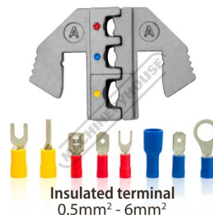
Insulated Terminal Jaw 0.5mm 2 - 6mm 2
