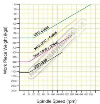
Work Piece Load Graph
