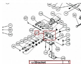
Parts Diagram
