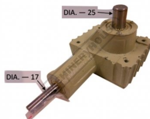
BD201 GEARBOX COMPLETE 18121 BD201 GEARBOX COMPLETE 18121 2
