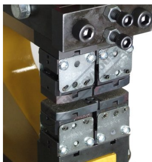
Reversible Jaws for Shinking and Stretching
