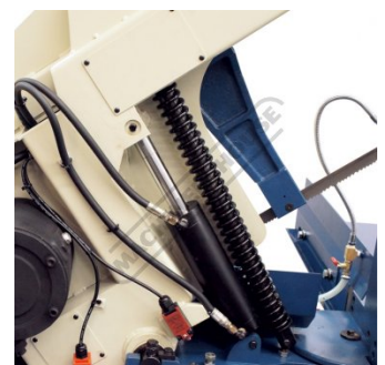
Hydraulic Rise-Fall with Spring Damper
