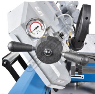
Blade Tension Gauge
