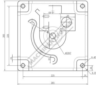
Base Dimensions
