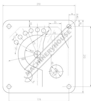
Base Dimensions
