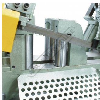
Feed Rolls
