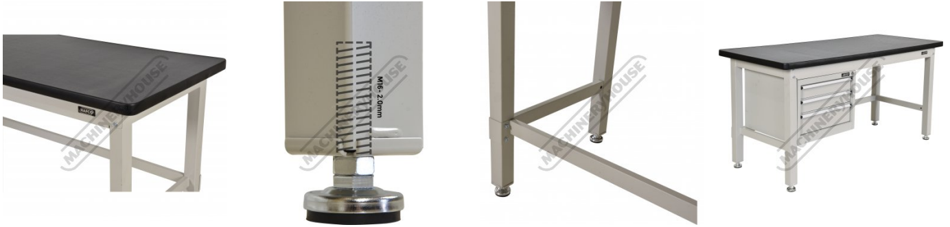
Rounded-bull nosed hard PVC edge Adjustable Feet - 16mm Internal thread Steel leg bracing Shown With Optional Draws A423
