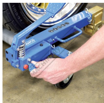
Closing Release Valve Ready for Pumping Jack
