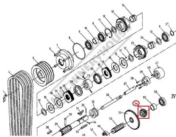
Headstock Assembly IV
