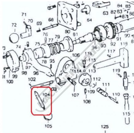
104 6234 Trip Handle
