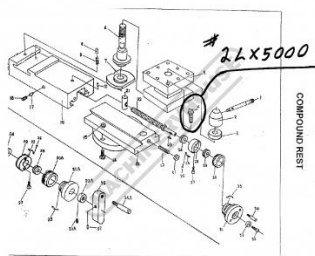
2LX5000 Assembly
