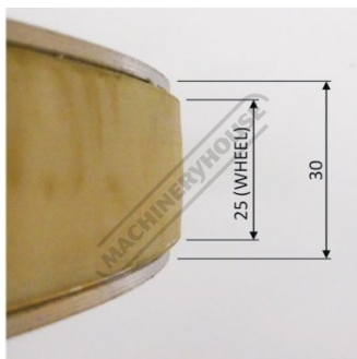
Wheel Outside Diameter 350 Bore (Bearing) 17 Close Up
