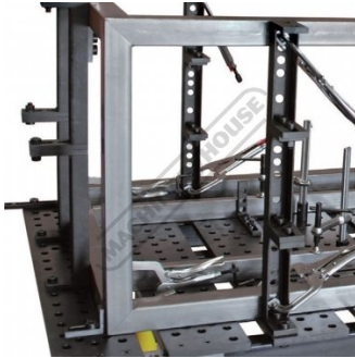
Stack Economy Stops as needed to Match the Height of Tall Workpieces or Fixtures
