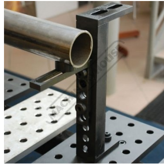
Add Modular Fixturing Components such as Rick Angle Brackets and V Blocks
