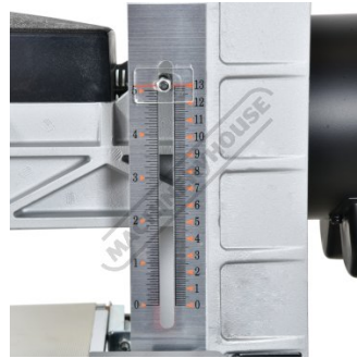
Height Gauge
