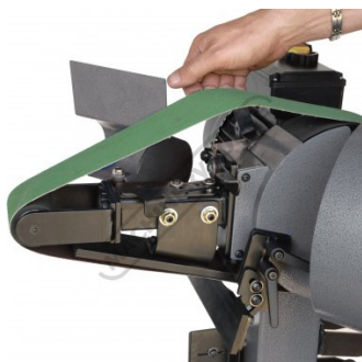
Belt Tension
