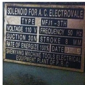
2DN1002 SOLENOID YA2 MFJ1 3TH
